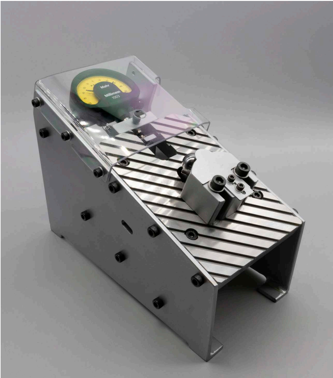
Evenness and depth machine for spherical track
